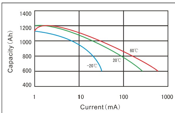
Capacity vs Current curve(cut off with 6.0V)
